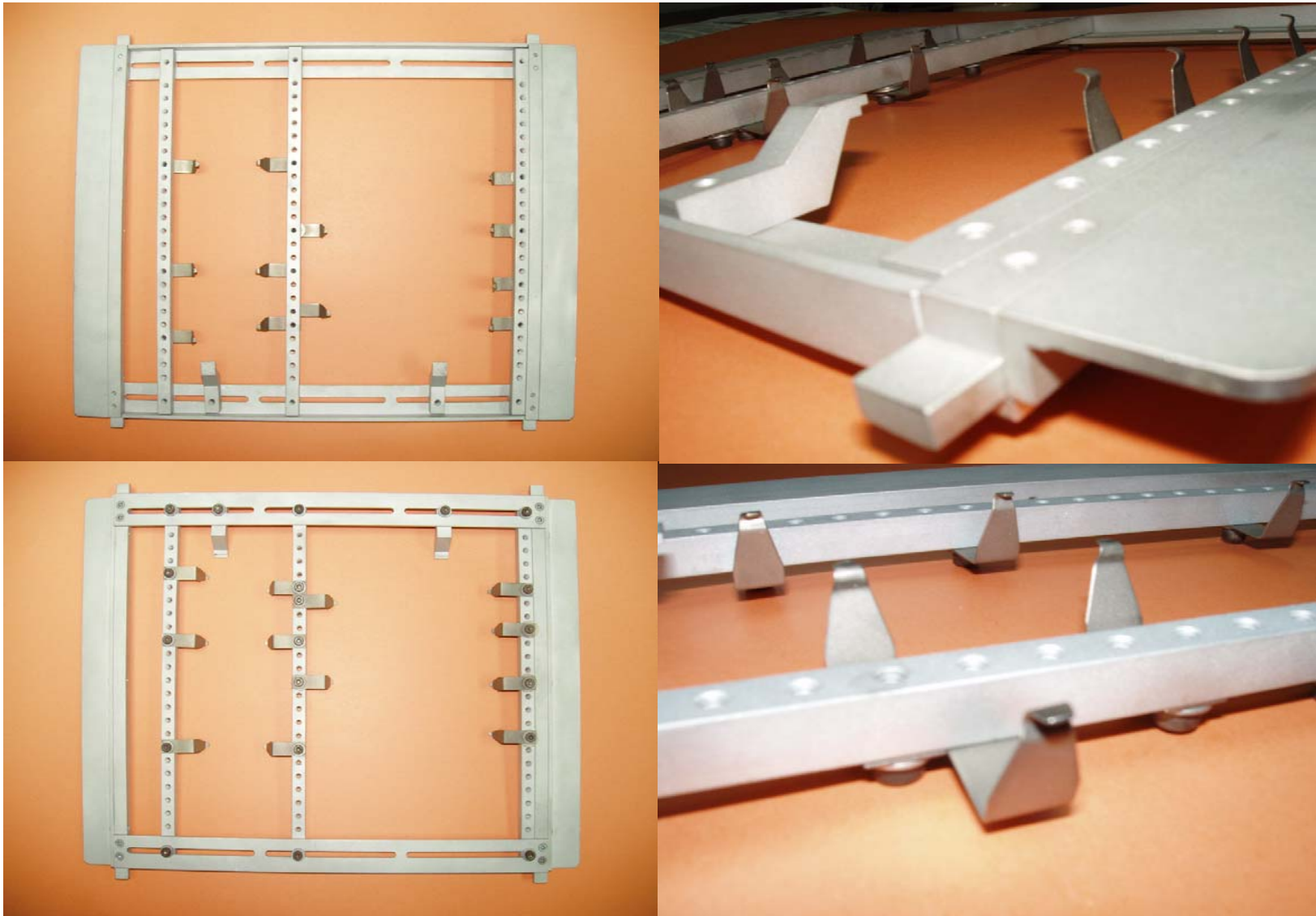
ADJUSTABLE PALLET FOR WAVE SOLDERING ALUMINIUM FRAME, STAINLESS STEEL BOLTS & TITANIUM FINGERS
