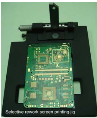
Selective rework screen printing jig
