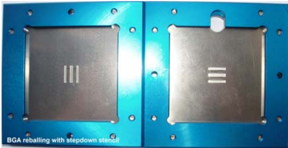
BGA reballing with stepdown stencil
