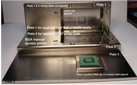
BGA manual screen printer
