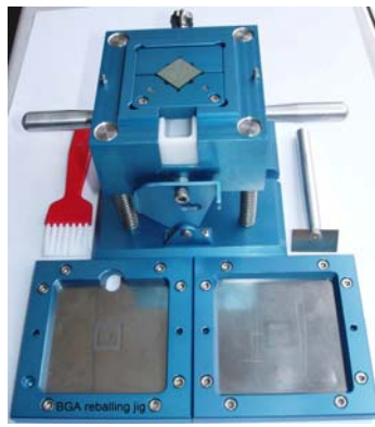
BGA reballing jig
