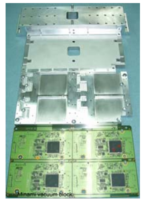
Minami vacuum block
